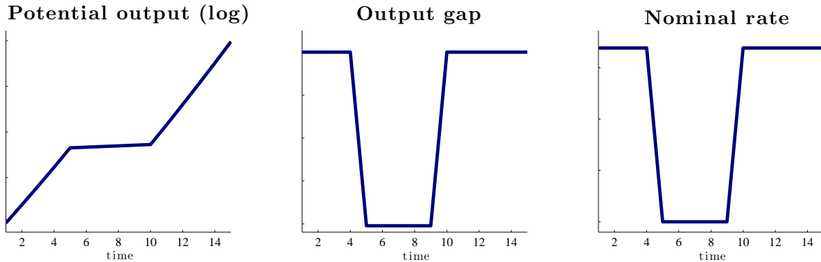
Figure 4: Dynamics around a temporary liquidity trap.
